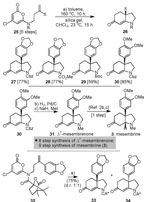
Scheme 2. Demonstration of the pyrone Diels–Alder approach through a total synthesis of \Delta^7 -mesembrenone ( 31 ), formal total synthesis of mesembrine ( 3 ), and a means to access enantiopure materials through a chiral auxiliary: a) toluene (0.02 M), 160 °C using microwave irradiation, 10 h, then CHCl 3 , silica gel, 23 °C, 15 h; b) 10% Pd/C (2.0 equiv), EtOAc, H 2 (1 atm), 23 °C, 3 h, quantitative; c) NaH (2.2 equiv), MeI (1.5 equiv), 23 °C, 45 min, 75% over two steps. Boc = tert -butoxycarbonyl, Cbz = carbobenzyloxy, CA* = chiral auxiliary; (1 S )-(–)-camphanoyl.
